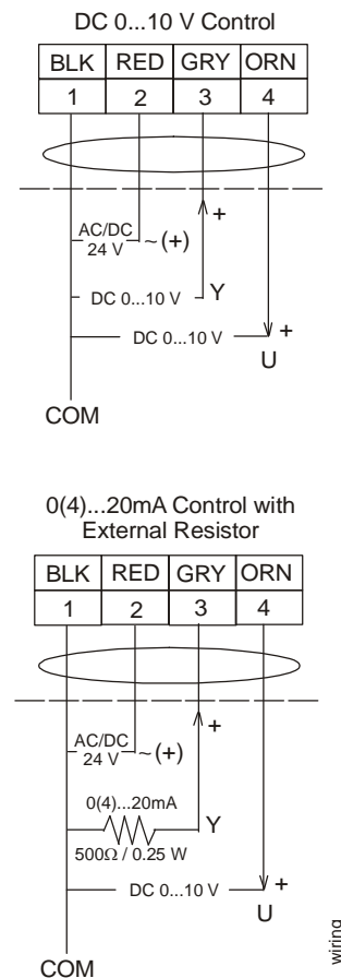
Figure 10: Control Wiring Diagrams
