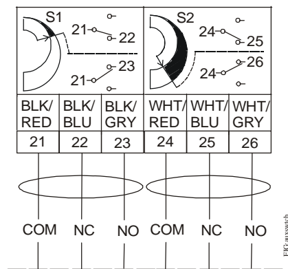
Figure 9: Auxiliary Switch Wiring Diagram for HGC Models
