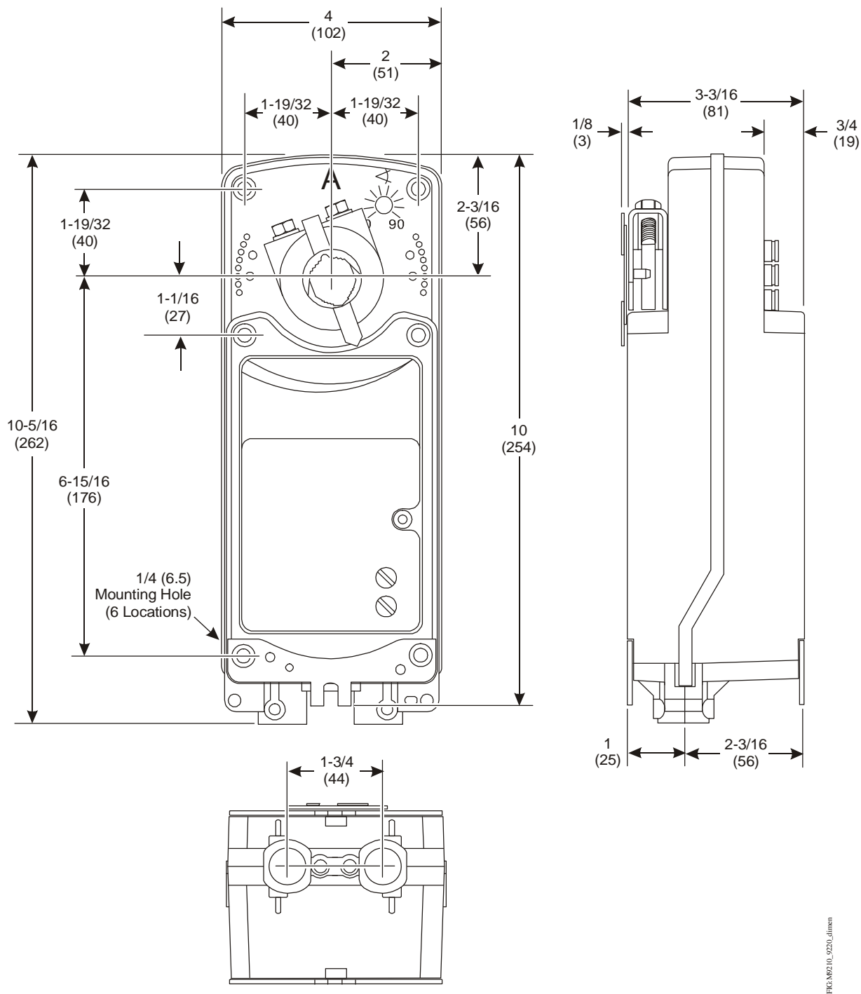
Figure 1: M9220-HGx-3 Proportional Electric Spring Return Actuator Dimensions, in. (mm)
