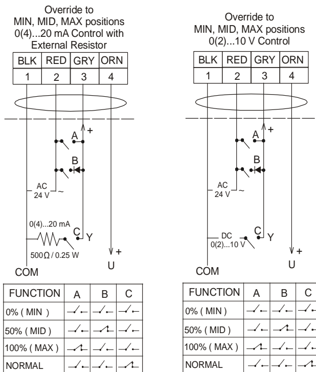
Figure 11: M9220-HGx-3 Control Wiring Diagram (Overrides)
