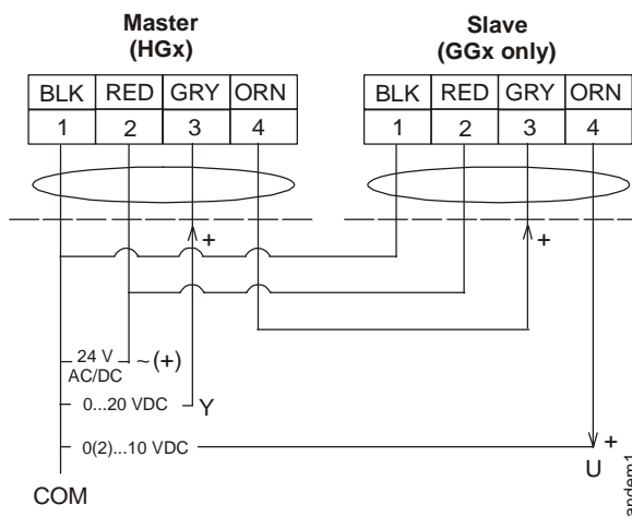
Figure 16: Tandem Connection
